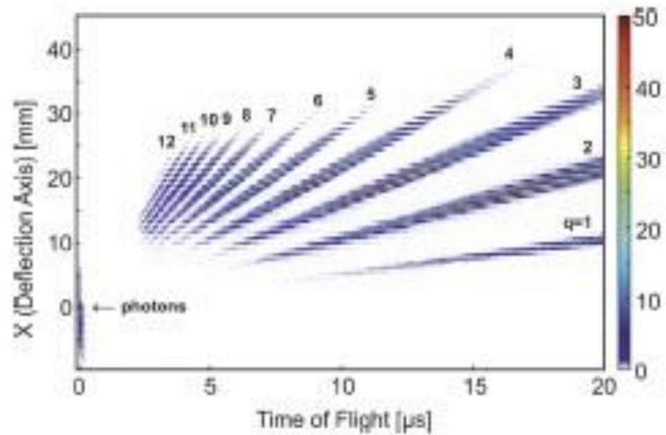
Time-resolved spatial histogram extracted from the data partially presented in Fig. 2. Each strip corresponds to a certain \text{Ag}^{q+} . Silver ion charge states up to q = 12 can clearly be distinguished. Events in the lower left corner of the spectrum stem from energetic photons. The ion yield is shown in arb. units as a color bar on the right hand side.
